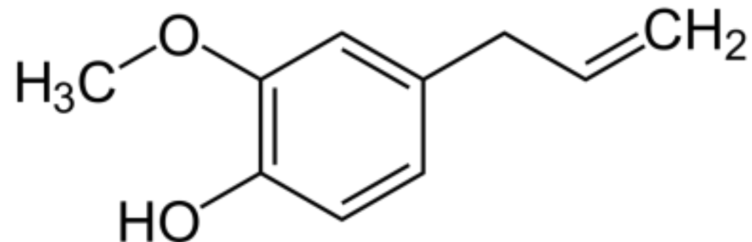
Eugenol
